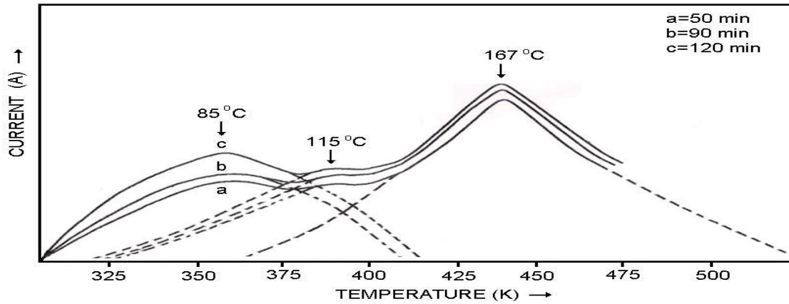
Fig.-1 : TSC Spectrum of acrylonitrile – isobornylacrylate
