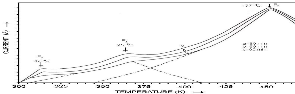
Fig.-2: TSC Spectrum of acrylonitrile – isobornylmethacrylate
