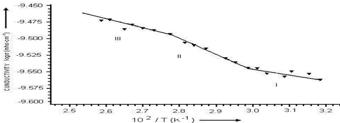
Fig. -4: Log \sigma Vs 1/T Plot for AN-IBA copolymer (I) (Probe spacing 0.8 cm)
