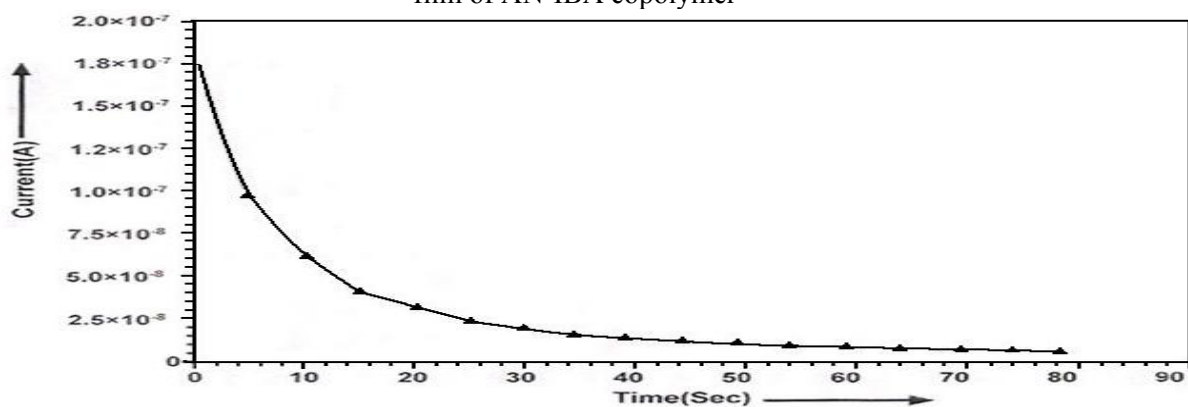
Fig.-7:Decay of current with time for potential applied to an irradiated (Voltage 120V) film of AN-IBA copolymer
