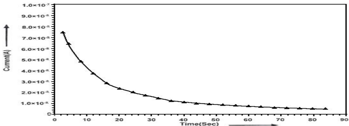
Fig.-6 :Decay of current with time for potential applied to the unirradiated (Voltage 120V) film of AN-IBA copolymer
