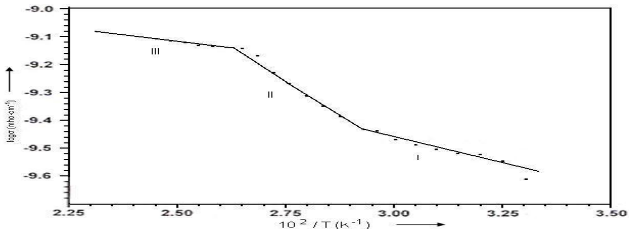
Fig.-9: Log \sigma Vs 1/T Plot for UV – irradiated AN-IBM copolymer (II) film
