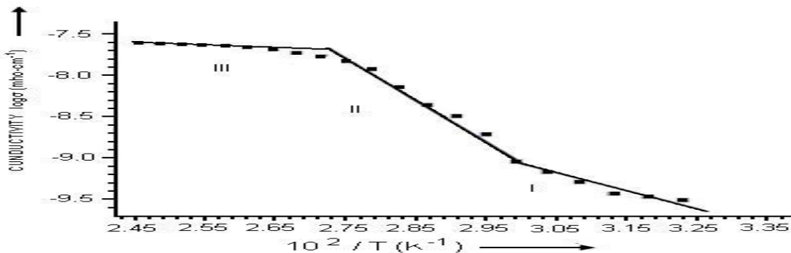
Fig.-3:Electrical conductivity ( \sigma ) Vs Temperature plot for (probe spacing 0.2 cm) AN-IBA copolymer(I)
