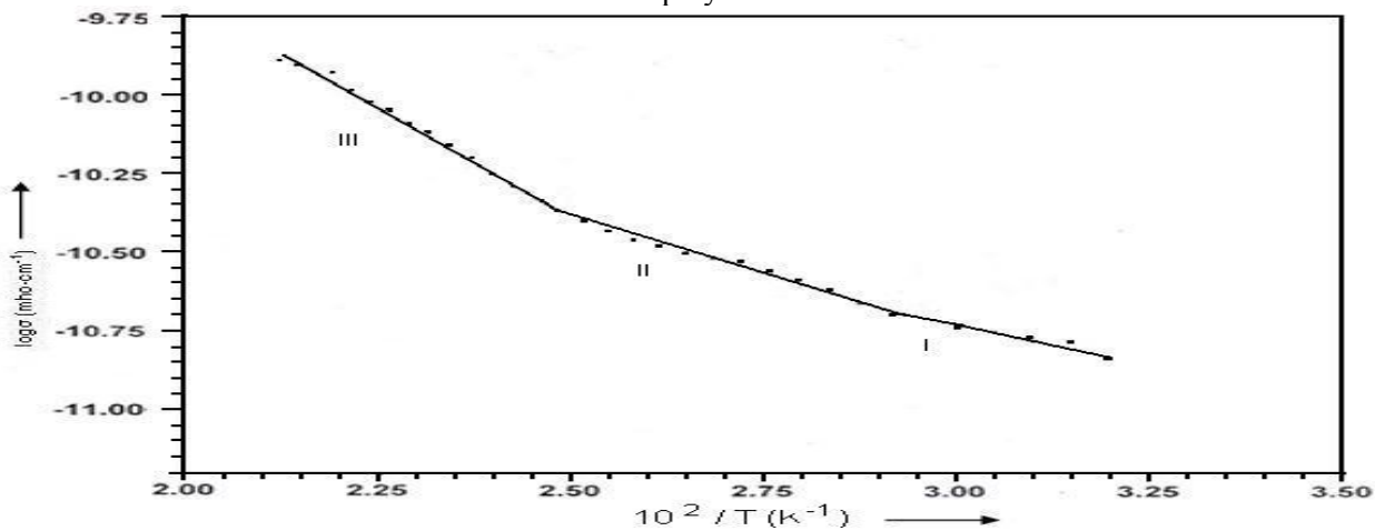
Fig.-8:Log \sigma Vs 1/T Plot for AN-IBM copolymer (II) (Probe spacing 0.8 cm)
