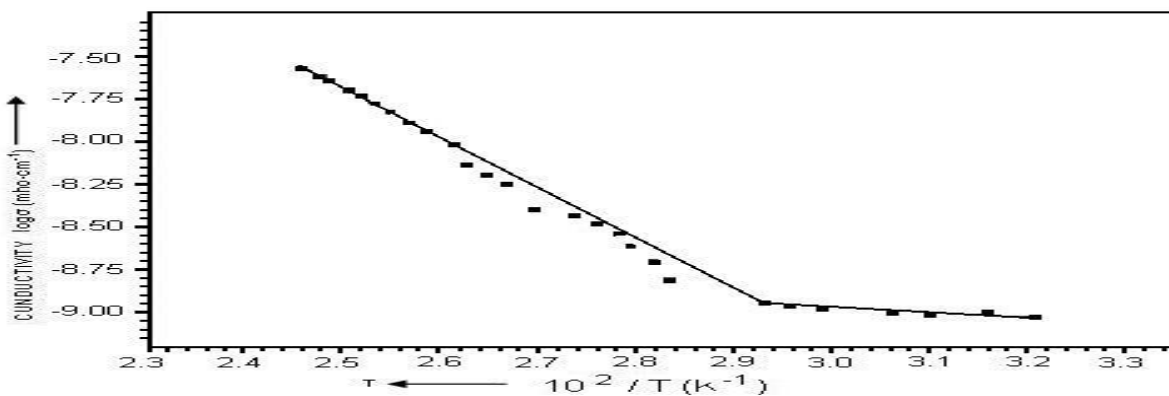
Fig-5 :Log \sigma Vs 1/T Plot for UV - irradiated AN-IBA copolymer
