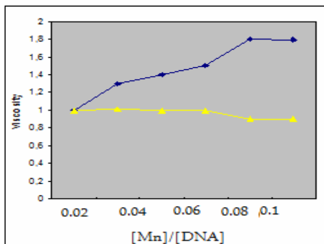
Fig.-4: Effect of increasing the amounts of [\text{Mn}(p\text{-H}_2\text{NC}_6\text{H}_4\text{COO})_2] \cdot 4\text{H}_2\text{O} (◆) on the relative (▲) viscosity of cat genomic DNA at 30.0 °C.
