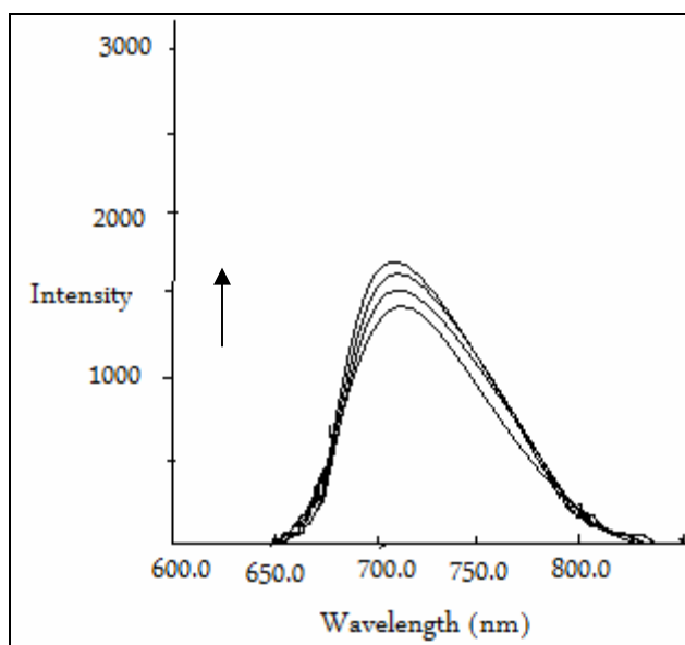
Fig.-2: Fluorescence spectra of [\text{Mn}(p\text{-H}_2\text{NC}_6\text{H}_4\text{COO})_2]4\text{H}_2\text{O} with increasing the concentration of genomic DNA.
