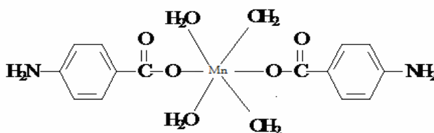
Fig.-1: The Structure of [Mn(p\text{-}H_2N\text{-}C_6H_4COO)_2]4H_2O complex.
