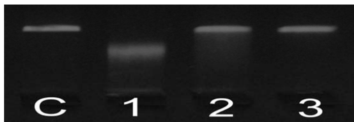
Fig.-3: Agarose gel electrophoresis diagram of cat genomic DNA- [\text{Mn}(p\text{-H}_2\text{NC}_6\text{H}_4\text{COO})_2] \cdot 4\text{H}_2\text{O} . Lane C: untreated cat genomic DNA, Lanes 1–3: DNA + [\text{Mn}(p\text{-H}_2\text{NC}_6\text{H}_4\text{COO})_2] \cdot 4\text{H}_2\text{O} complex in the concentration of 10, 1, 0.1 mM.
