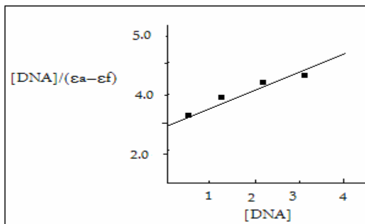
Fig.-6: Plots of [\text{DNA}]/(\epsilon_a - \epsilon_f) versus [\text{DNA}] for the titration of DNA with the complex
