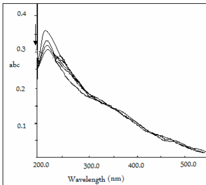
Fig.-5: Electronic spectra of [\text{Mn}(p\text{-H}_2\text{NC}_6\text{H}_4\text{COO})_2]4\text{H}_2\text{O} (10 mM) in the presence of increasing amounts of genomic DNA ( [\text{DNA}] = 0\text{--}25 mM). The arrow indicates the absorbance changes on increasing DNA concentration.
