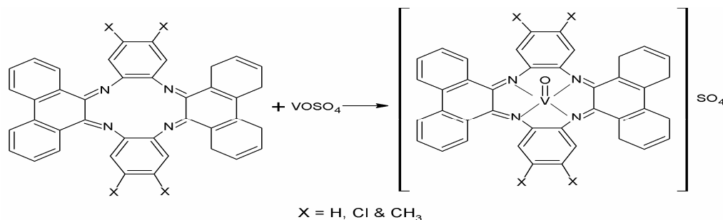
Fig.-2: Synthesis of macrocyclic Schiff base complexes
