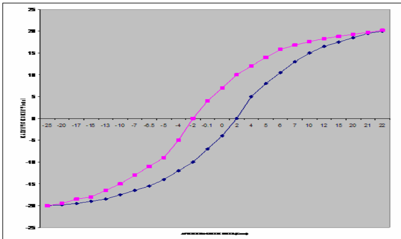
Fig.-3: Magnetic hysteresis loop of sample -1, (X= 0), System Cu_{1-x} Cd_x [Fe_{1-x} Al_x Cr_{1-x} Mn_x]O_4
