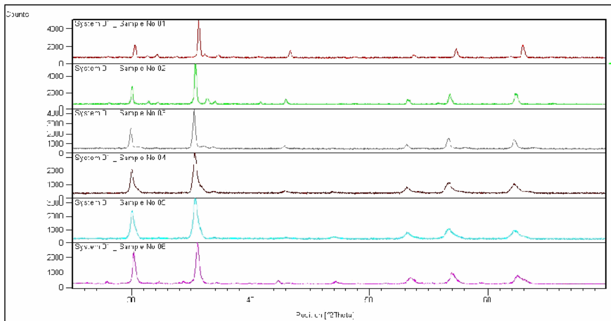
Fig.-1: X- Ray diffractometer pattern of System Cu_{1-x} Cd_x [Fe_{1-x} Al_x Cr_{1-x} Mn_x]O_4
