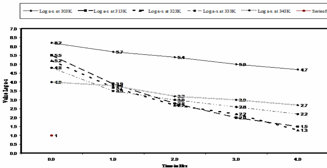
Fig.-4 :Catalytic Parameters of sample – 1, (X = 0), System Cu_{1-x} Cd_x [Fe_{1-x} Al_x Cr_{1-x} Mn_x]O_4
