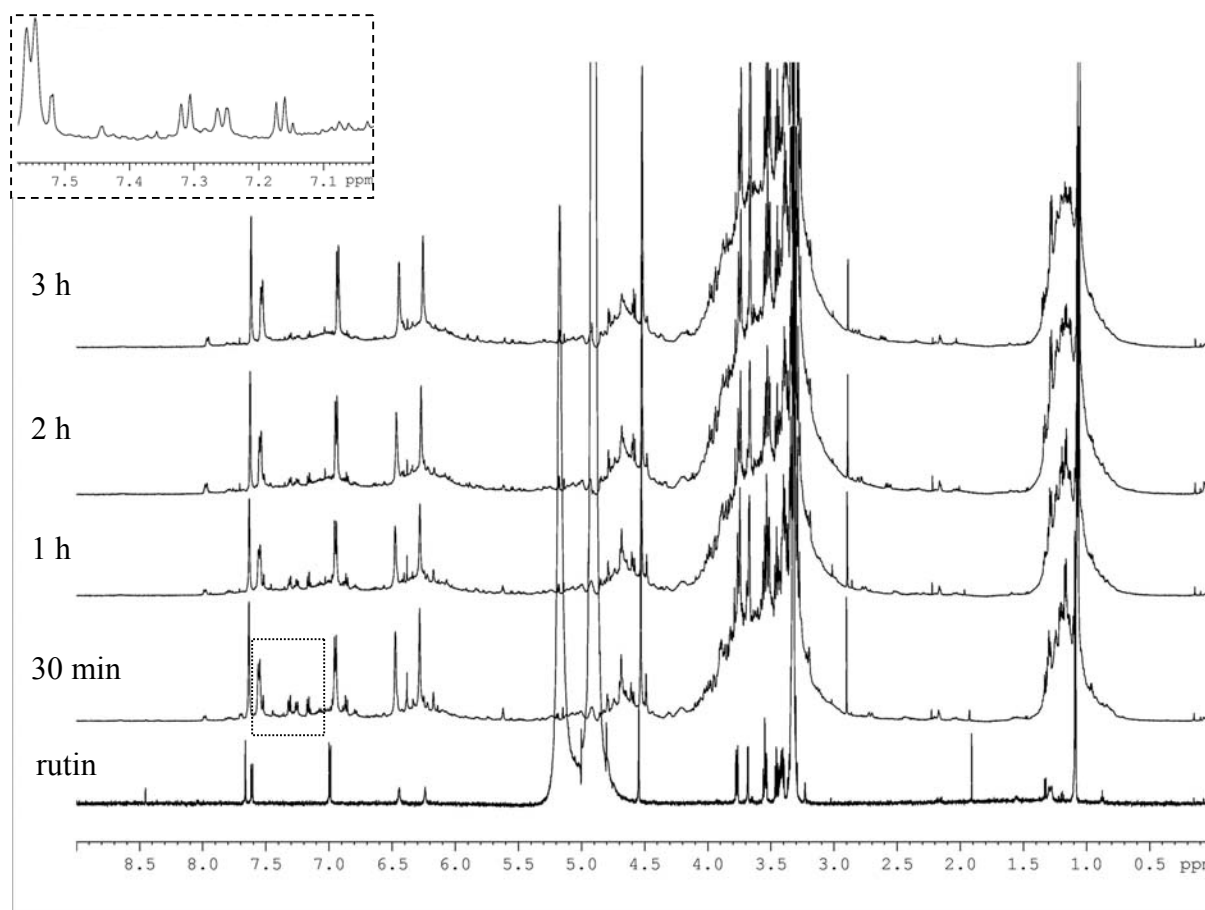
Figure-6: ^1\text{H-NMR} (600 MHz by cryoprobe) spectra of media containing rutin and oligomers of rutin at four times (30 min, 1 h, 2 h, 3 h) of reaction. Rutin (0.2 g/L) oligomerization was catalyzed by the laccase from Trametes versicolor (0.3 U/mL) in \text{CD}_3\text{OD}/\text{D}_2\text{O} (30:70, v/v), at 20 °C.
