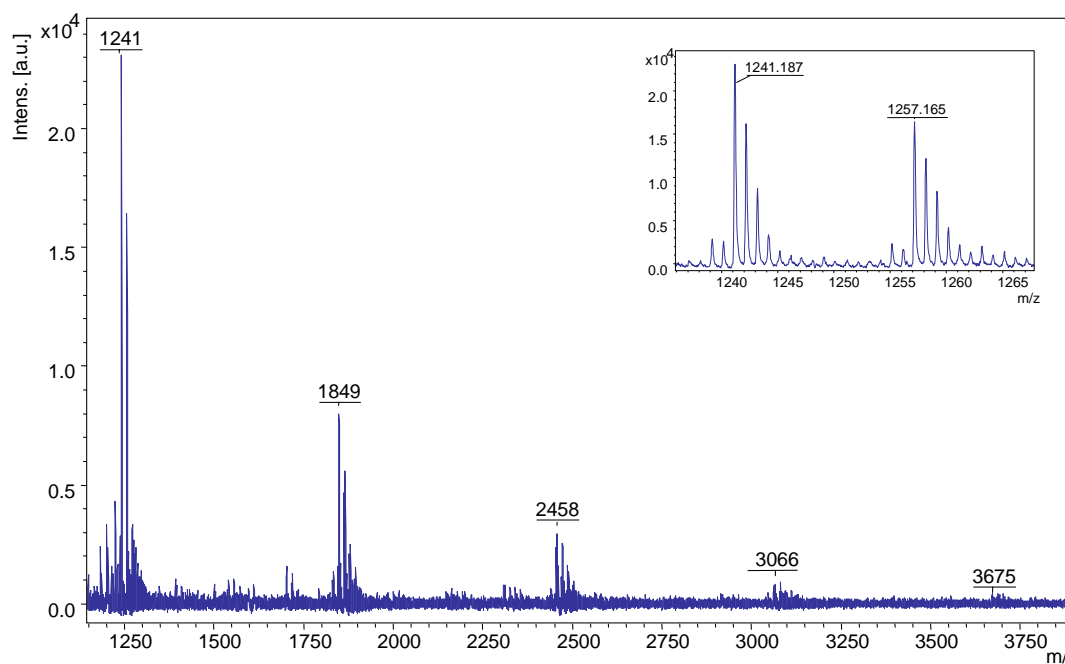
Figure-4: MALDI-TOF positive ion spectrum ( [M - H + Na \text{ or } K]^+ ) in the reflectron mode of rutin oligomerization media and isotopic distribution of dimer. Dihydroxybenzoic acid was used as matrix.
